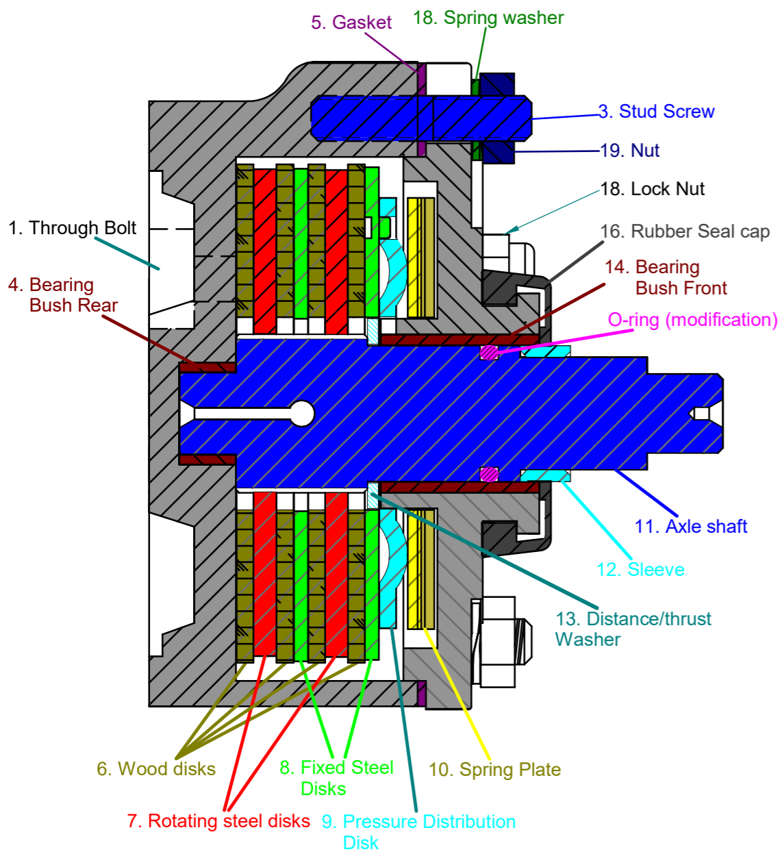
SIDE VIEW
